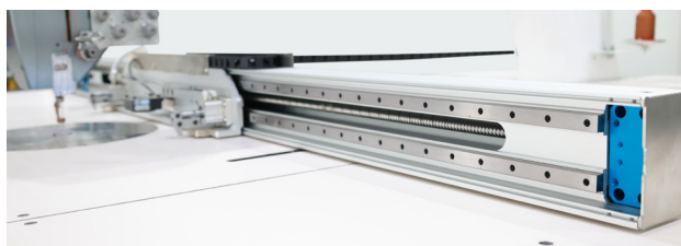
上银导轨、TBI丝杆 HIWIN Linear Guide Rails, TBI Ball Screws
